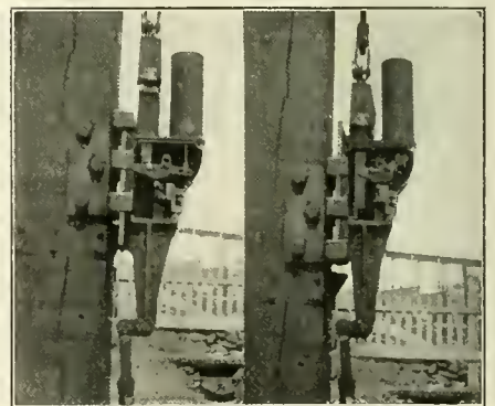
TWO POSITIONS OF ELECTRIC SLOT MECHANISM ON SIGNAL AT ENTRANCE OF BERGEN TUNNEL, ERIE.
